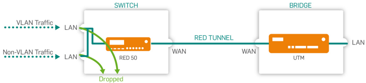
Figure 28 LAN mode: Disabled
