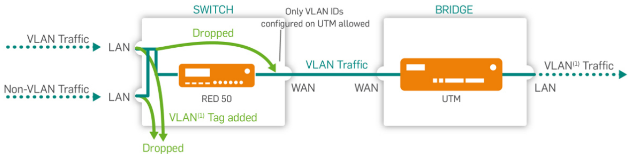
Figure 27 LAN mode: Tagged
