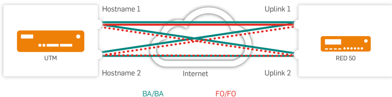
Figure 29 RED 50: Hostname and Uplink Balancing (turquoise) and Hostname and Uplink Failover (red)
